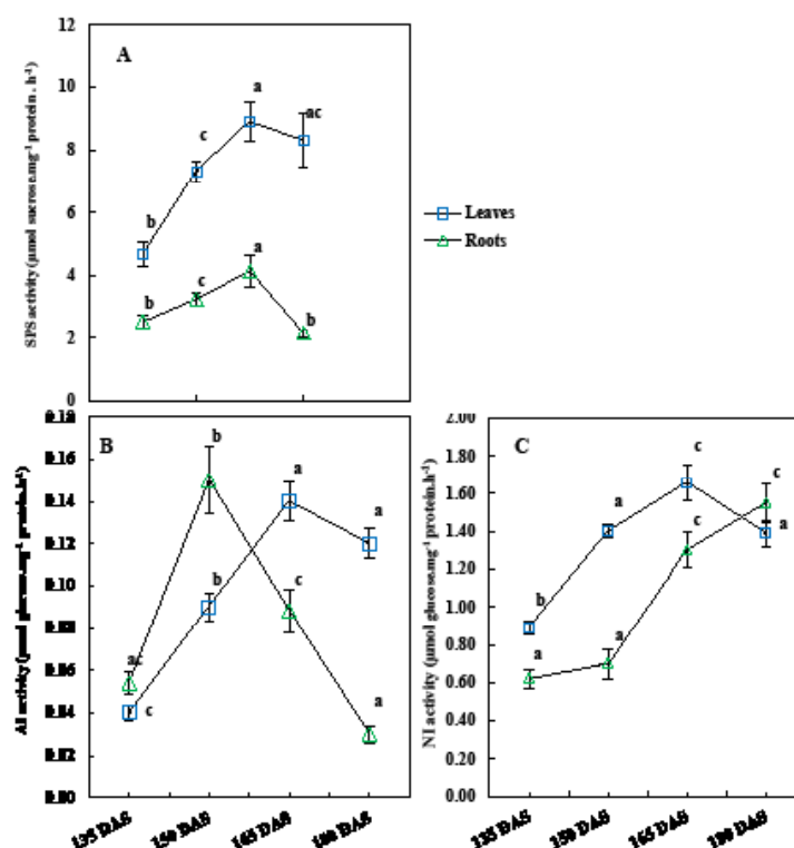
Fig. 2. Changes in activity of sucrose metabolism enzymes: A, SPS; B, AI and C, NI in leaves and roots of sugar beet plants during different developmental phases. Values are means \pm SE (n = 3). Different letters indicate a significant variance at P \leq 0.05 , LSD test.
