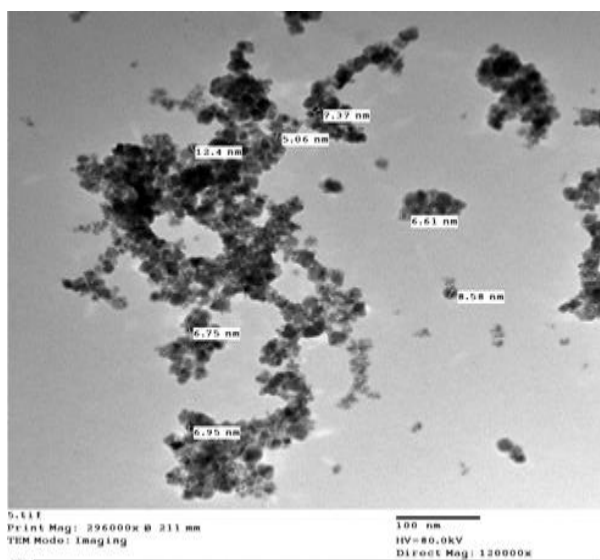
Fig. 1. TEM images and size distribution of titanium dioxide nanoparticle.
