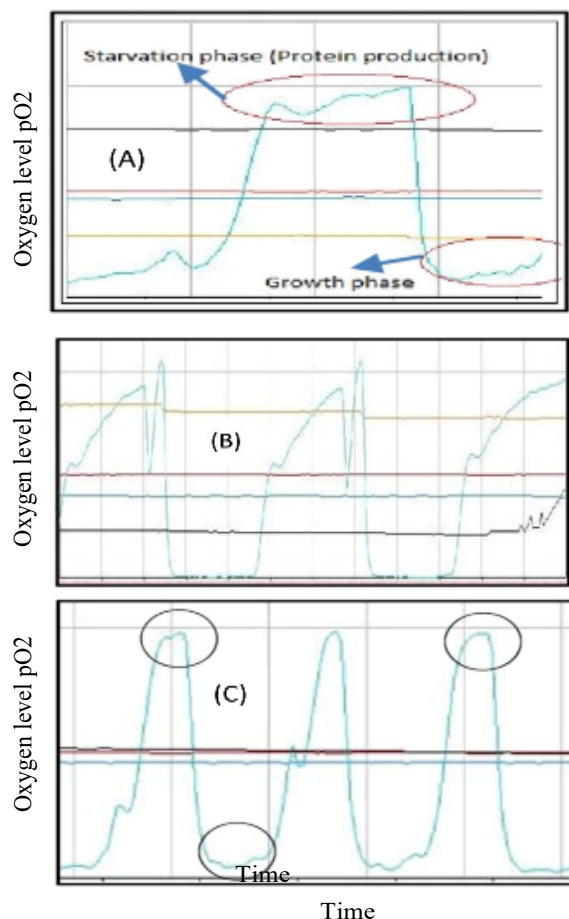
Figure 4. Impact of different addition shots of glycerol, during H. polymorpha growth-protein expression phase, on po2 level vs time: (A) 600 gm/shot showed long starvation period, (B) 700 gm/shot, (C) 500gm/shot showed short starvation period.
