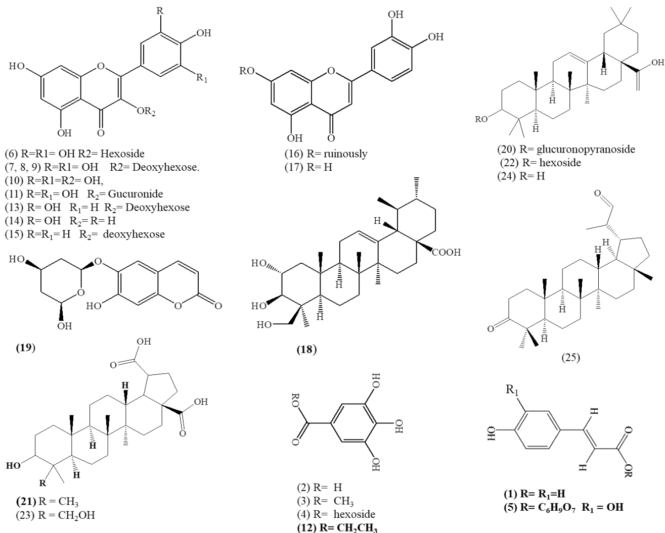
Figure 7. Basic structures of the 25 phytochemical compounds that have been tentatively identified from the aqueous fraction by LC ESI-MS/MS analysis : (1) p-coumaric acid, (2) gallic acid, (3) methyl gallate, (4) O-galloylglucose, (5) caffeoyl glucaric acid isomers, (6) myricetin-3-O-β-D-hexoside, (7, 8, 9) Myricetin O-deoxyhexose, (10) Myricetin, (11) myricetin -O-glucuronide, (12) ethyl gallat, (13) quercetin -O- rhamnoside, (14) quercetin, (15) Kaempferol -O rhamnoside, (16) Luteolin- O –rutinoside, (17) Luteolin (18) 2a, 3a, 24-trihydroxyurs-12-en-28-oic acid, (19) Esculin, (20) oleanolic acid-O-glucuronylpyranosyl, (21) Hydroxy betulinic acid, (22) Oleanolic acid 3-O-α-glycoside, (23) betulinic acid, (24) Oleanolic acid, (25) (20S)-3-Oxolupan-30-al.
